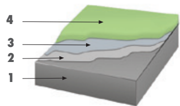
MAPEFLOOR SYSTEM 53 TRASPIRANTE 2 - 4 mm
